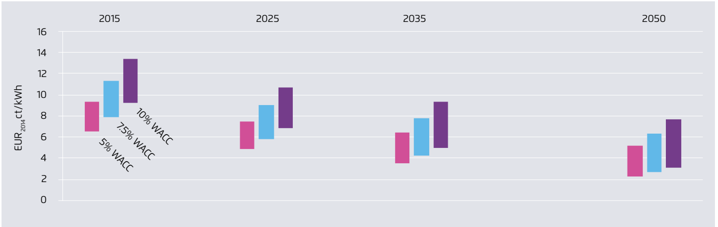
LCOE South Africa (1000 - 1300 kWh/kWp p.a.); WAAC between 5% and 10%
