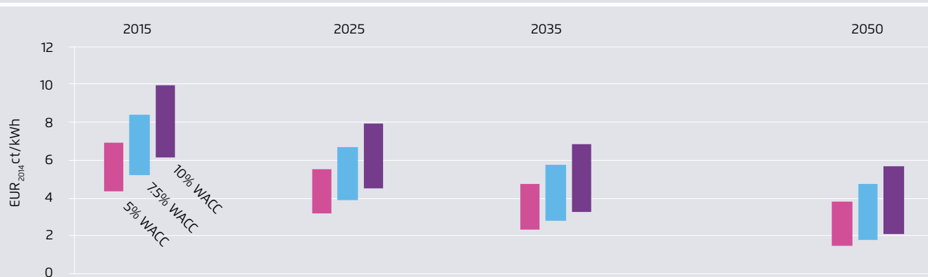
LCOE United States (1350 - 1950 kWh/kWp p.a.); WAAC between 5% and 10%
