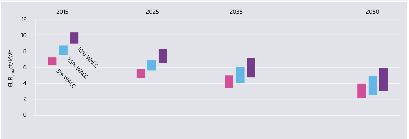
LCOE Korea, South (1300 - 1350 kWh/kWp p.a.); WAAC between 5% and 10%
