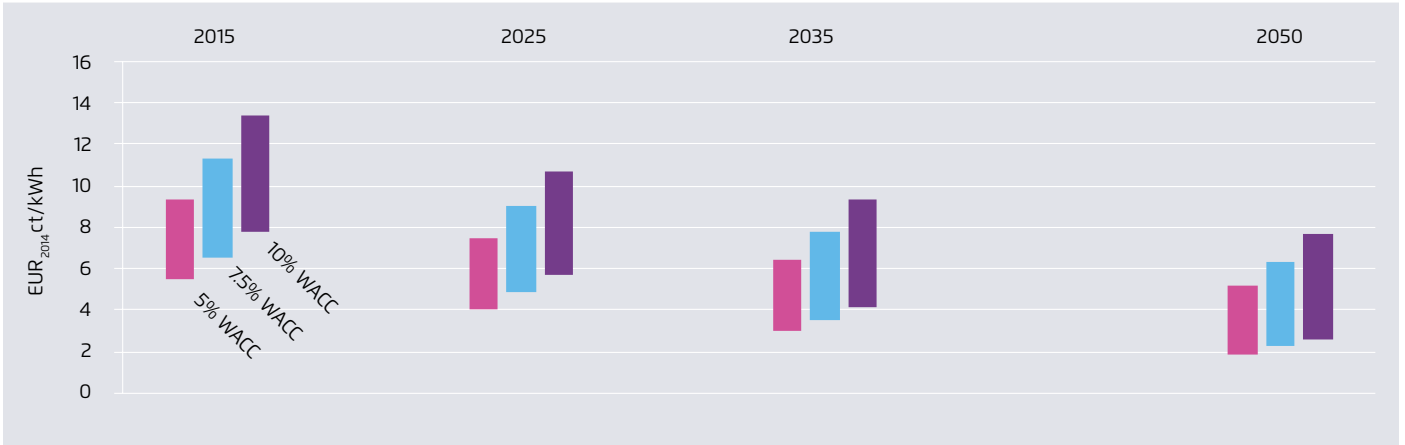
LCOE France (1000 - 1550 kWh/kWp p.a.); WAAC between 5% and 10%
