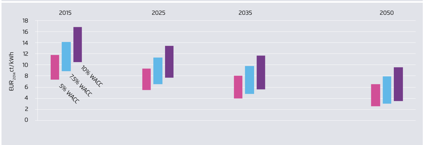
LCOE United Kingdom (800 - 1150 kWh/kWp p.a.); WAAC between 5% and 10%
