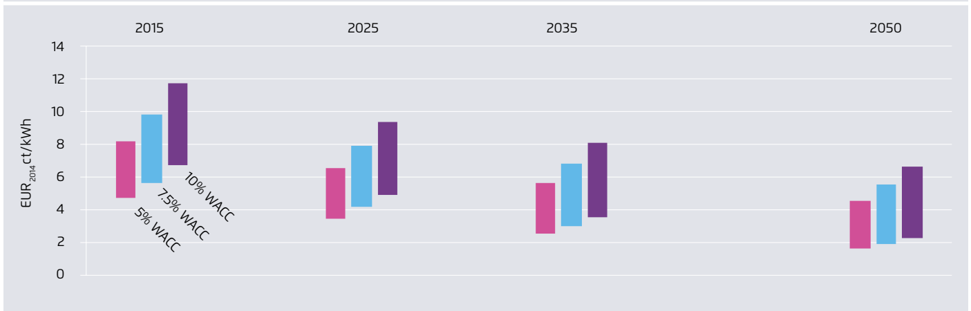
LCOE Brazil (1150 - 1800 kWh/kWp p.a.); WAAC between 5% and 10%
