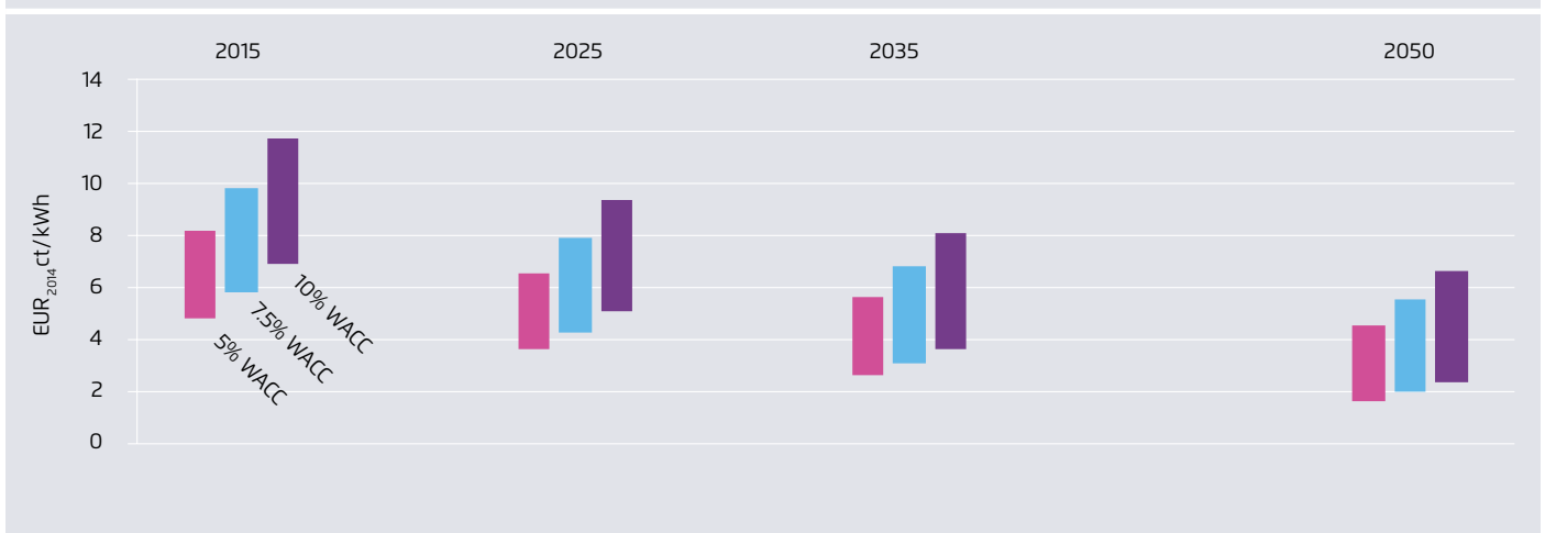
LCOE China (1150 - 1750 kWh/kWp p.a.); WAAC between 5% and 10%
