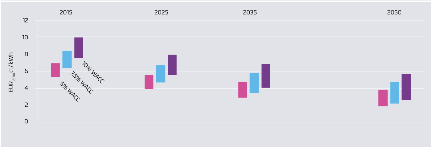
LCOE Thailand (1350 - 1600 kWh/kWp p.a.); WAAC between 5% and 10%
