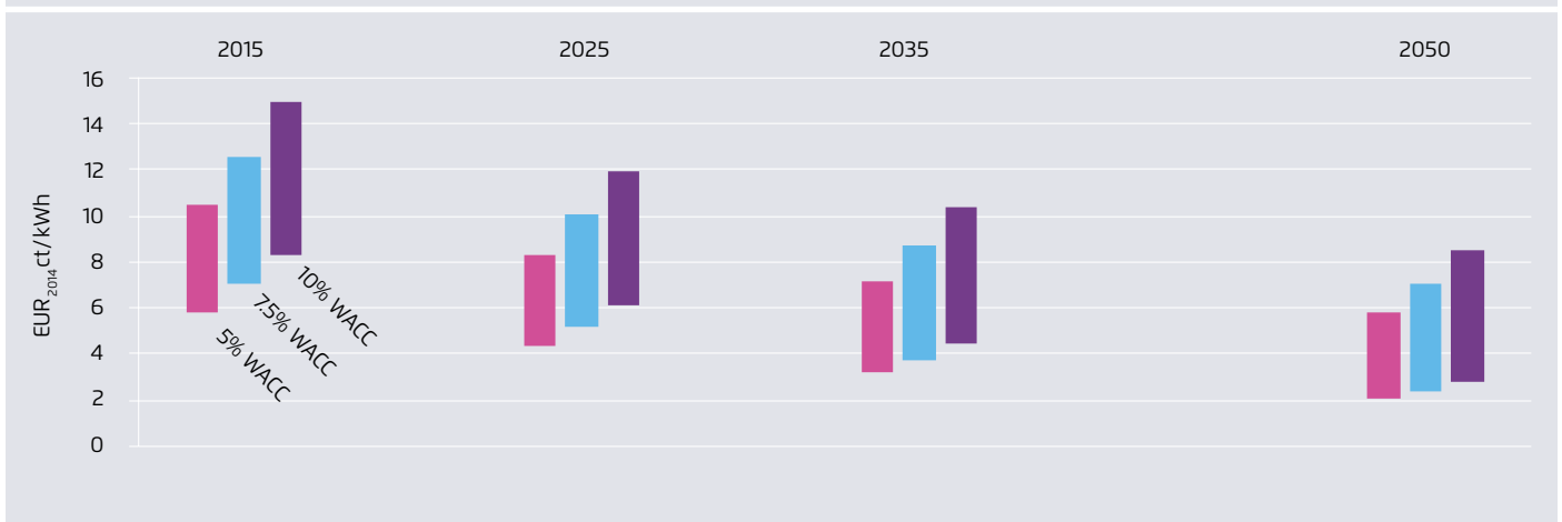
LCOE Canada (900 - 1450 kWh/kWp p.a.); WAAC between 5% and 10%
