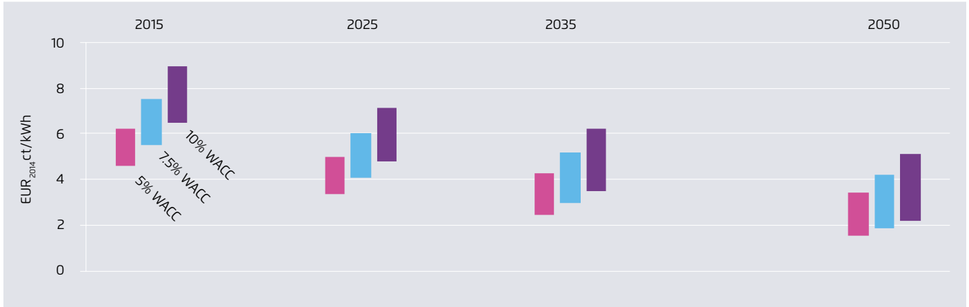
LCOE Morocco (1500 - 1850 kWh/kWp p.a.); WAAC between 5% and 10%
