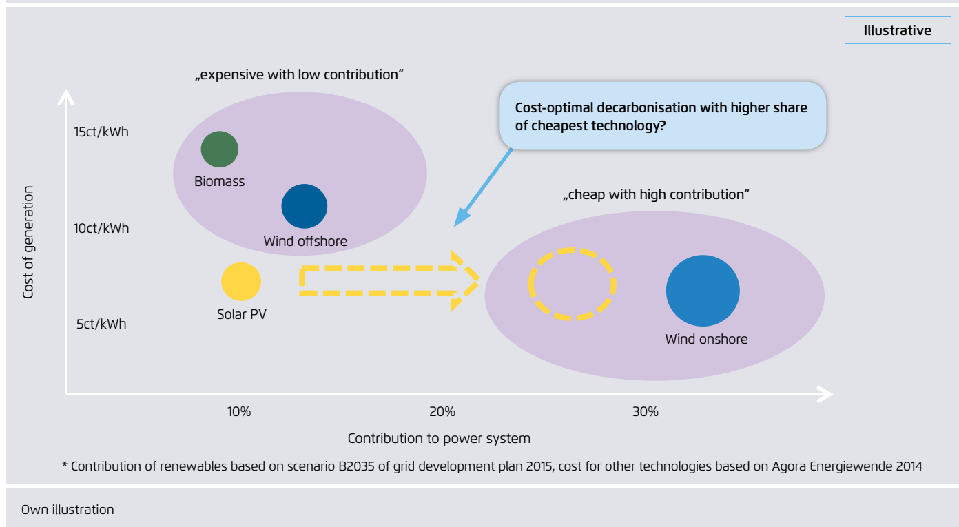
Cost of generation and contribution to power system per technology, in Germany in 2035*
