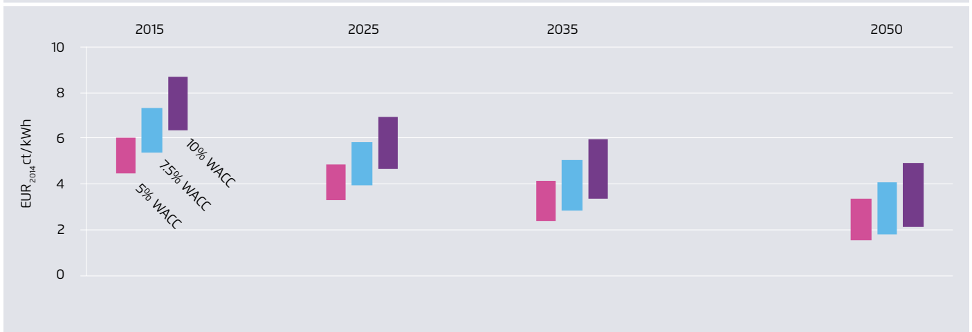
LCOE Saudi Arabia (1550 - 1900 kWh/kWp p.a.); WAAC between 5% and 10%
