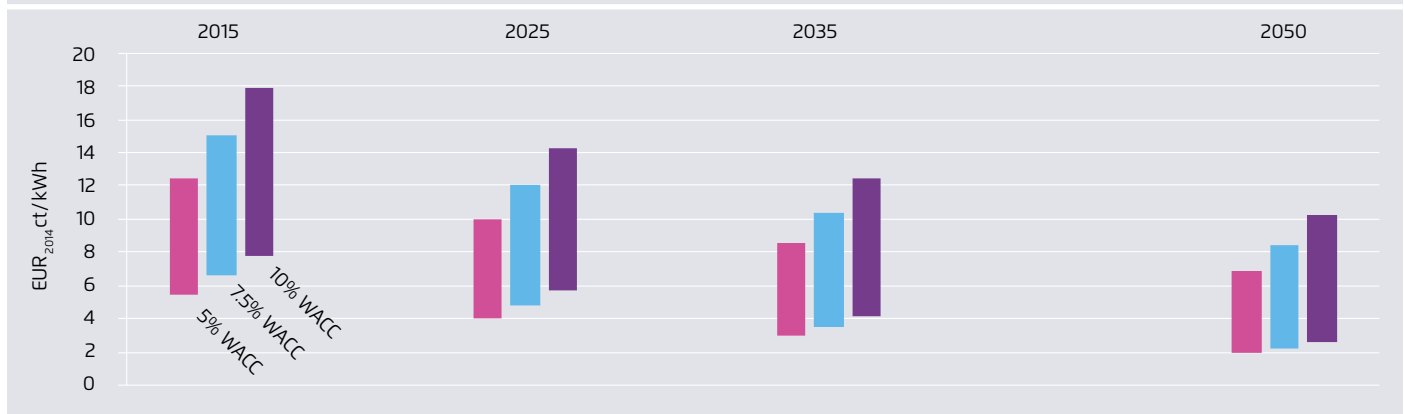
LCOE Australia (1050 - 1850 kWh/kWp p.a.); WAAC between 5% and 10%
