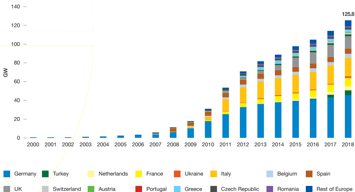
FIGURE 33 EUROPEAN TOTAL SOLAR PV INSTALLED CAPACITY 2000-2018
