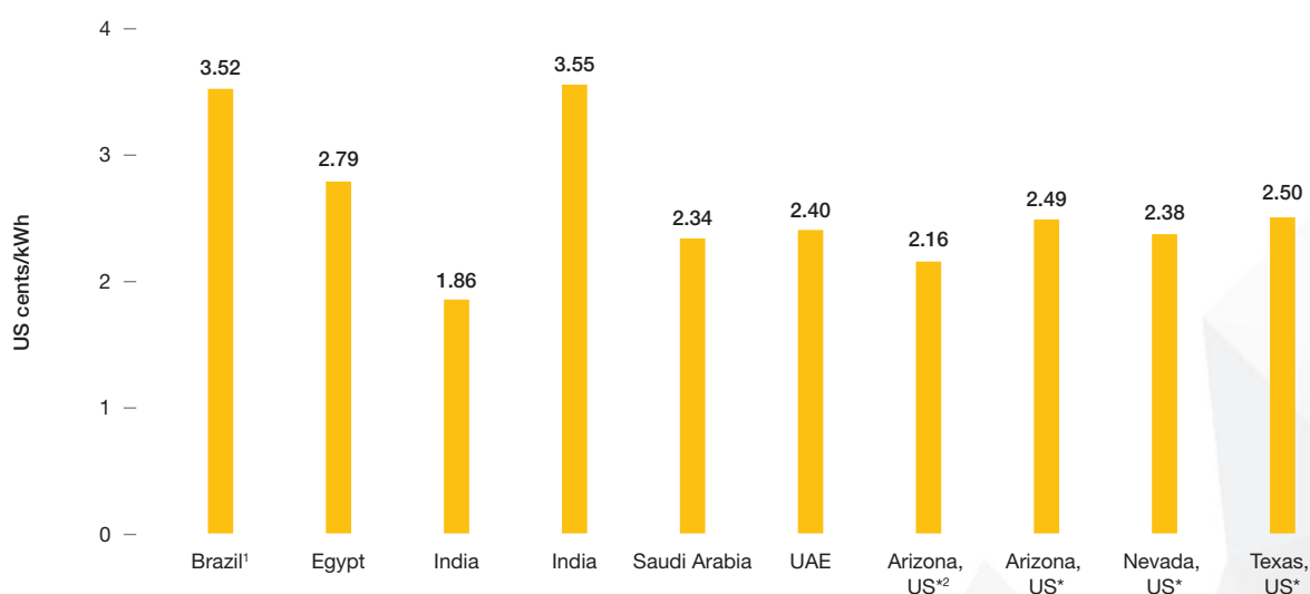
FIGURE 4 SELECTION OF LOWEST SOLAR AUCTION BIDS AROUND THE WORLD IN 2018
