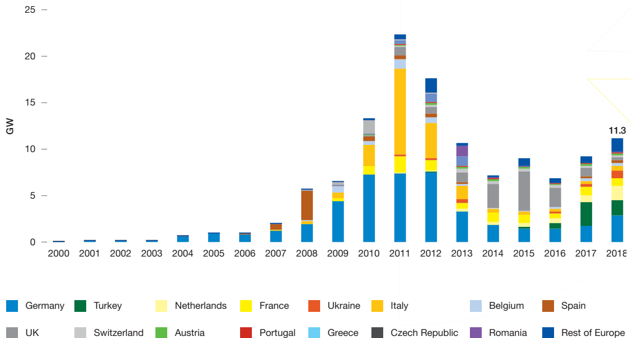
FIGURE 32 EUROPEAN ANNUAL SOLAR PV INSTALLED CAPACITY 2000-2018
